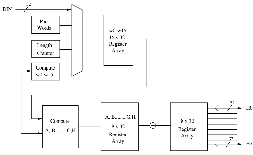
Figure 1: Block Diagram for the SHA-256 processor
